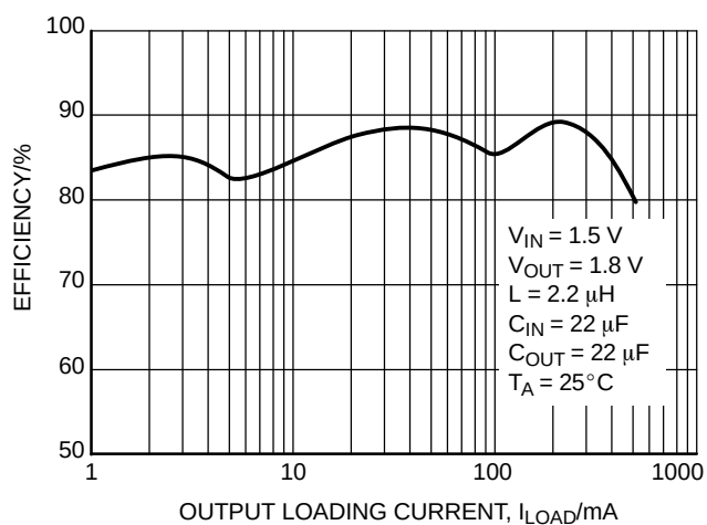
Figure 13. Efficiency vs. Load Current
