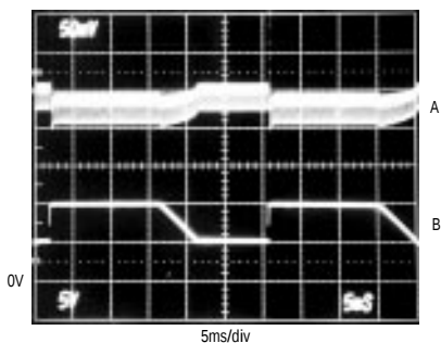
LINE-TRANSIENT RESPONSE
