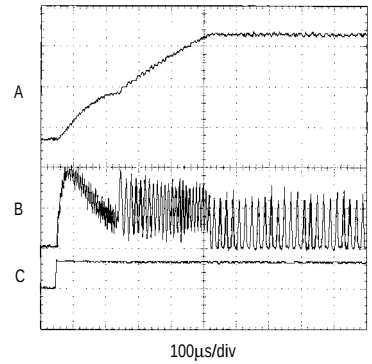
POWER-UP RESPONSE
