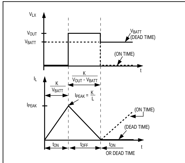
Figure 2. Switching Waveforms
