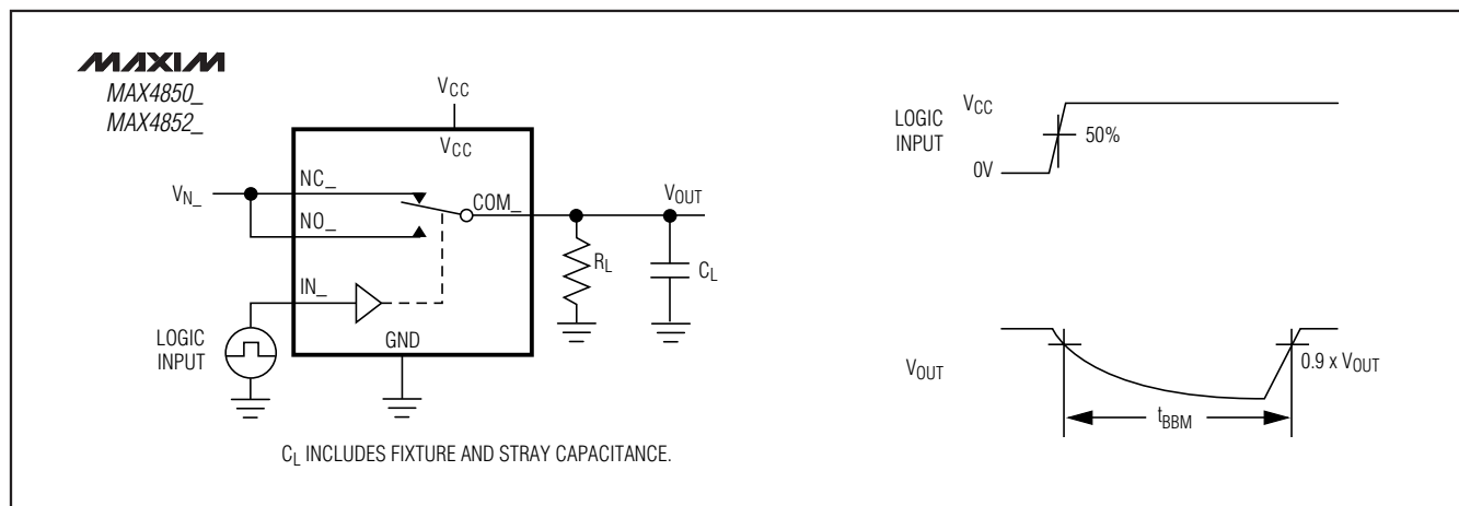
Figure 3. Break-Before-Make Interval
