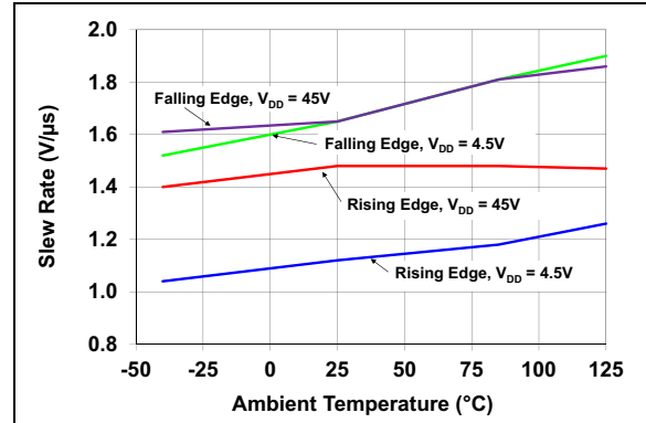
FIGURE 2-44: Slew Rate vs. Ambient Temperature.
