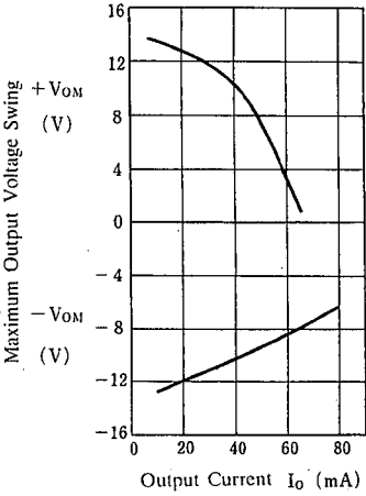
Maximum Output Voltage Swing
