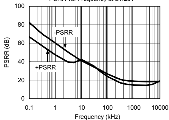
PSRR vs. Frequency at ±1.25V
