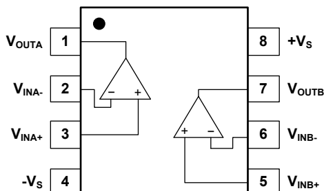
SGM8040-2 (TOP VIEW)
