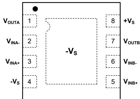
TDFN-2x2-8L
