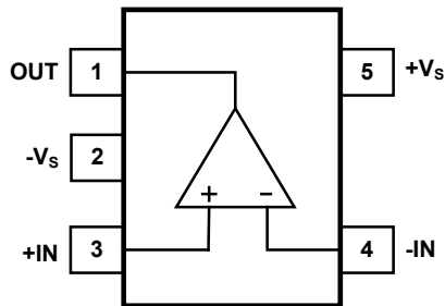
SGM8631 (TOP VIEW)
