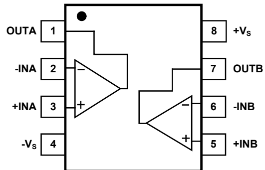
SGM8632 (TOP VIEW)
