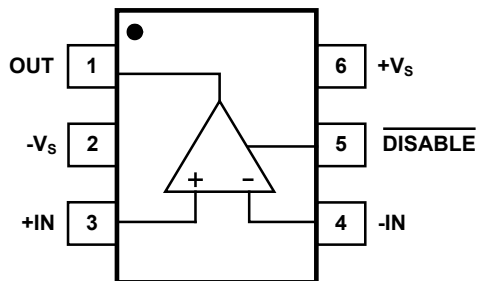
SGM8633 (TOP VIEW)
