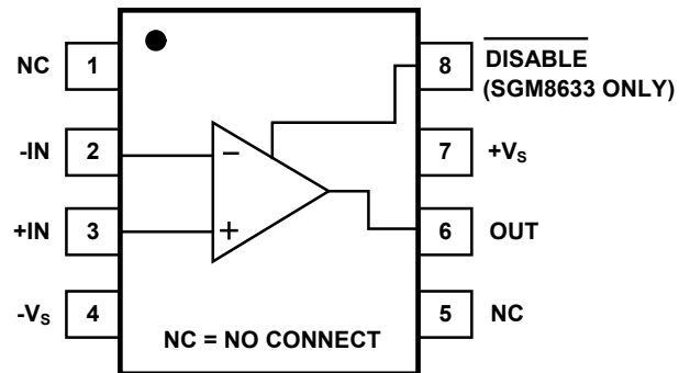
SGM8631/8633 (TOP VIEW)
