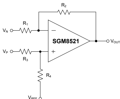
Figure 4. Differential Amplifier
