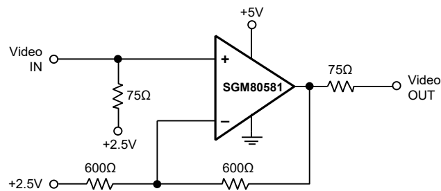
Figure 4. Single-Supply Video Line Driver
