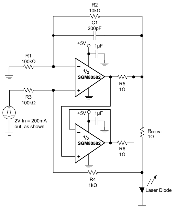
Figure 3. Parallel Operation
