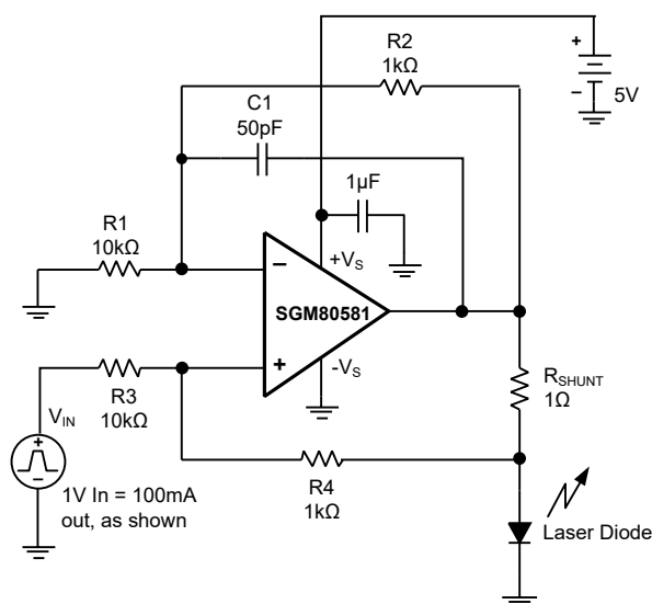
Figure 2. Laser Diode Driver
