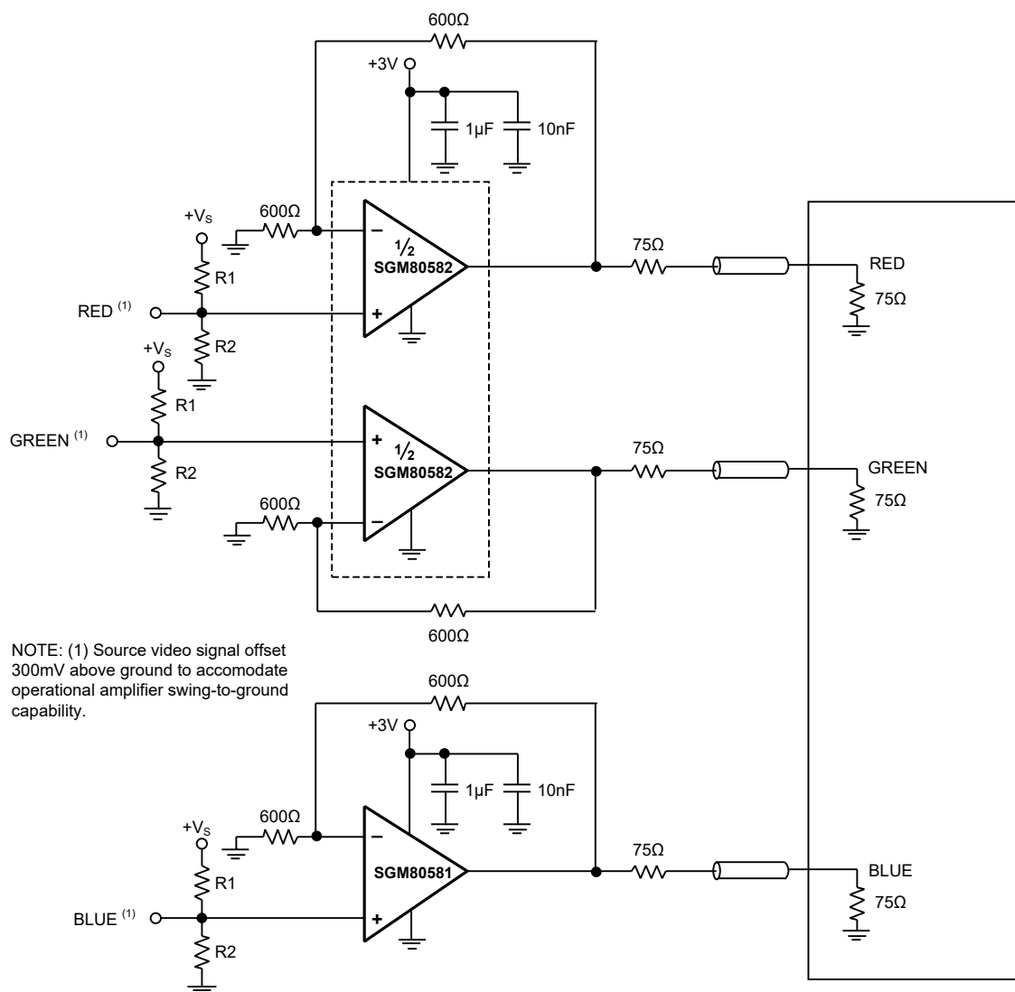
Figure 5. RGB Cable Driver
