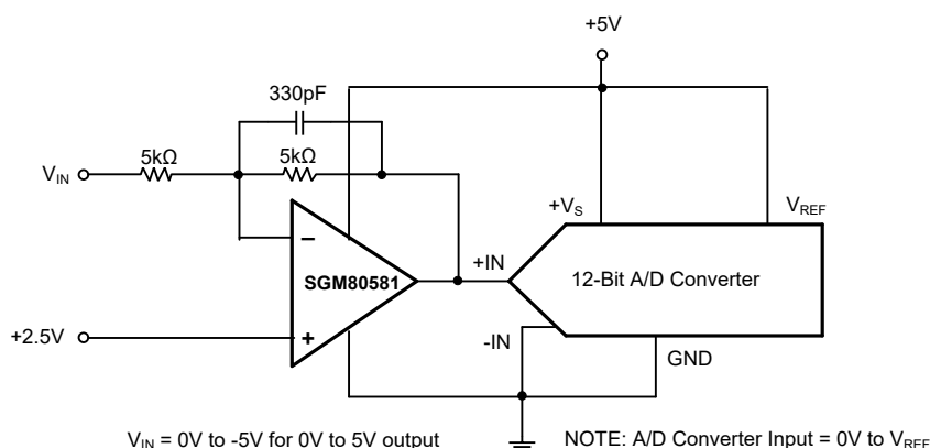
Figure 6. The SGM80581 in Inverting Configuration Driving an ADC
