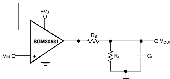
Figure 7. Series Resistor in Unity-Gain Configuration Improves Capacitive Load Drive
