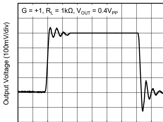
Non-Inverting Small-Signal Step Response
