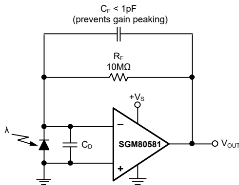
Figure 8. Transimpedance Amplifier
