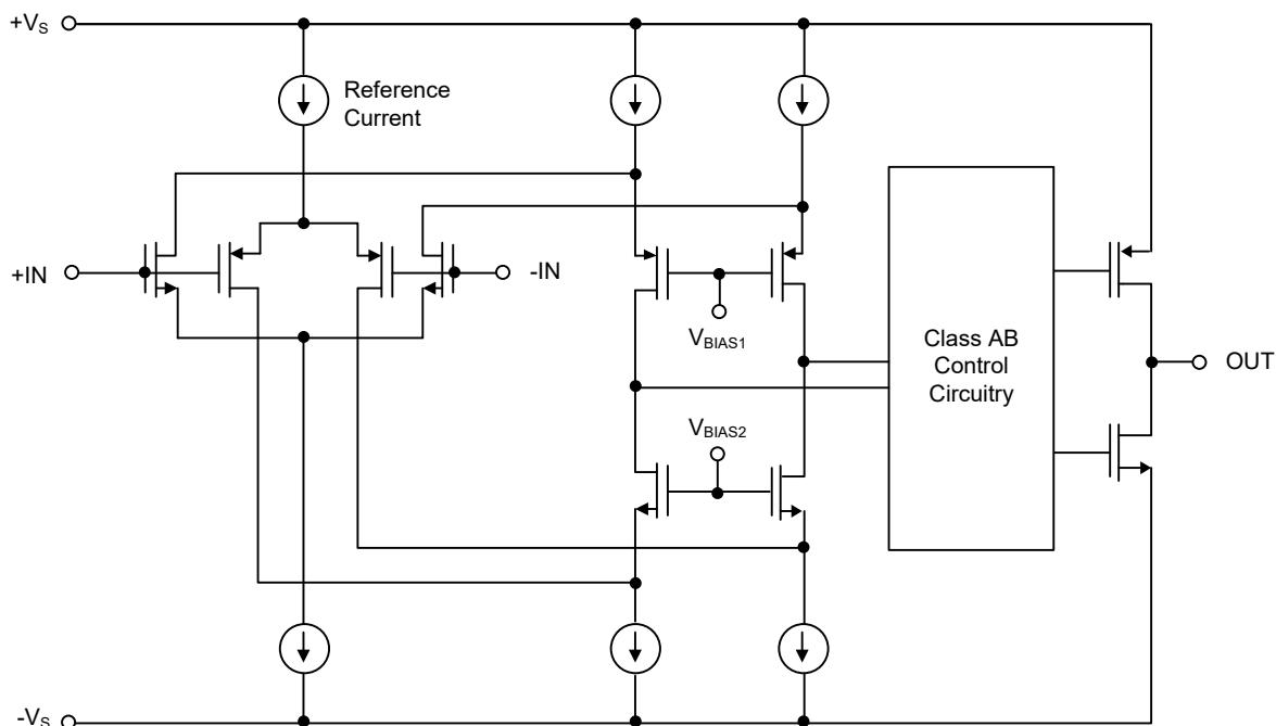
Figure 1. Simplified Schematic
