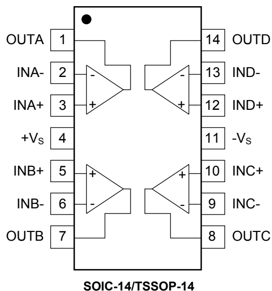
SGM8304 (TOP VIEW)
