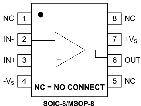
SGM8301 (TOP VIEW)
