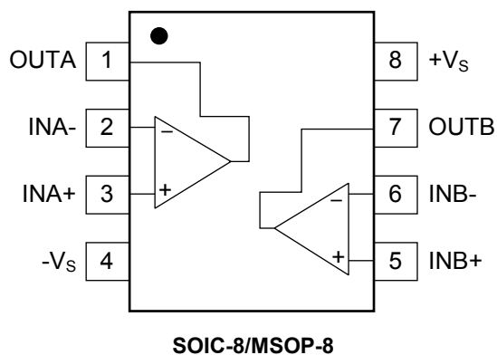
SGM8302 (TOP VIEW)
