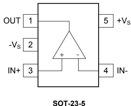
SGM8304 (TOP VIEW)
