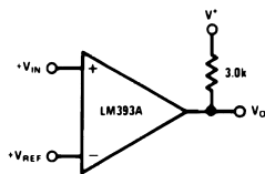
Basic Comparator
