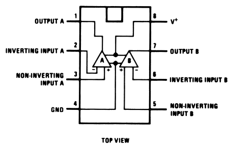
Dual-In-Line Package
