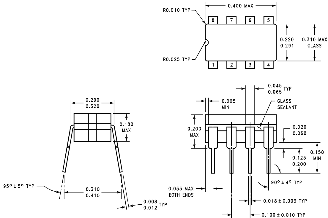
Order Number LM193J/883, LM193AJ/883, LM193AJ-MLS or LM193AM-MLS NS Package Number J08A
