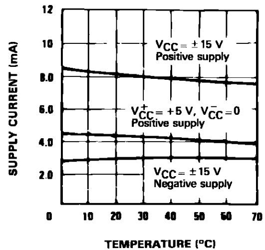
SUPPLY CURRENT
