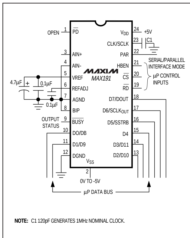
Figure 3. Operational Diagram
