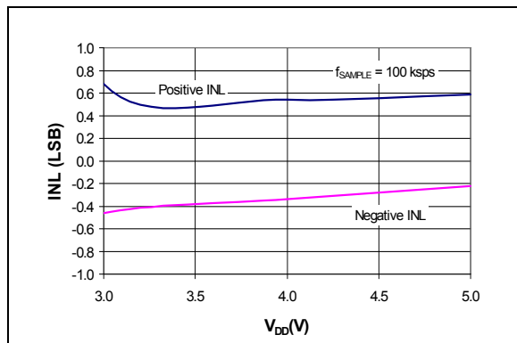
FIGURE 2-2: Integral Nonlinearity (INL) vs. V_{DD} .
