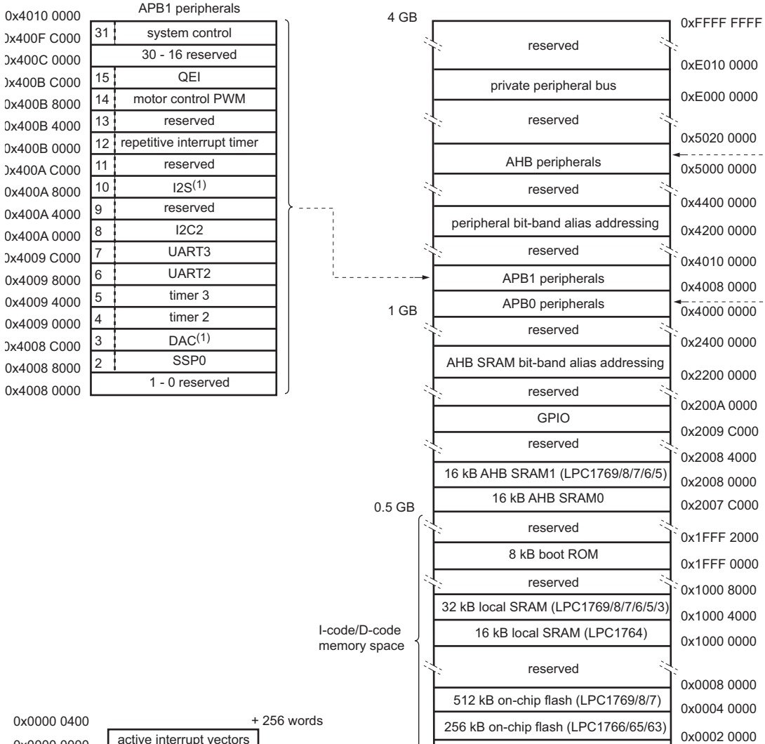
(1) Not available on all parts. See Table 2 . Fig 5. LPC17xx memory map
