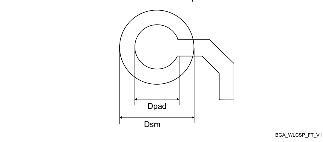
Figure 64. TFBGA - 100 balls, 8X8 mm, 0.8 mm pitch fine pitch ball grid array recommended footprint
