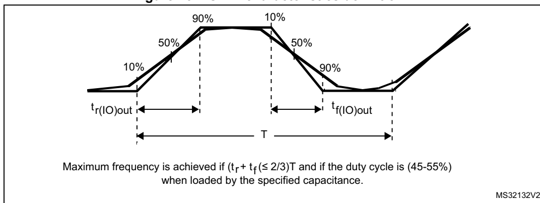
Figure 25. I/O AC characteristics definition (1)
