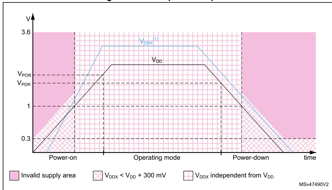
Figure 3. Power-up/down sequence
