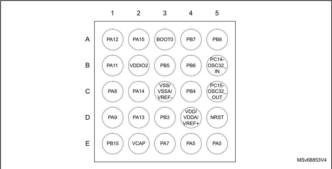
Figure 4. WLCSP25 pinout
