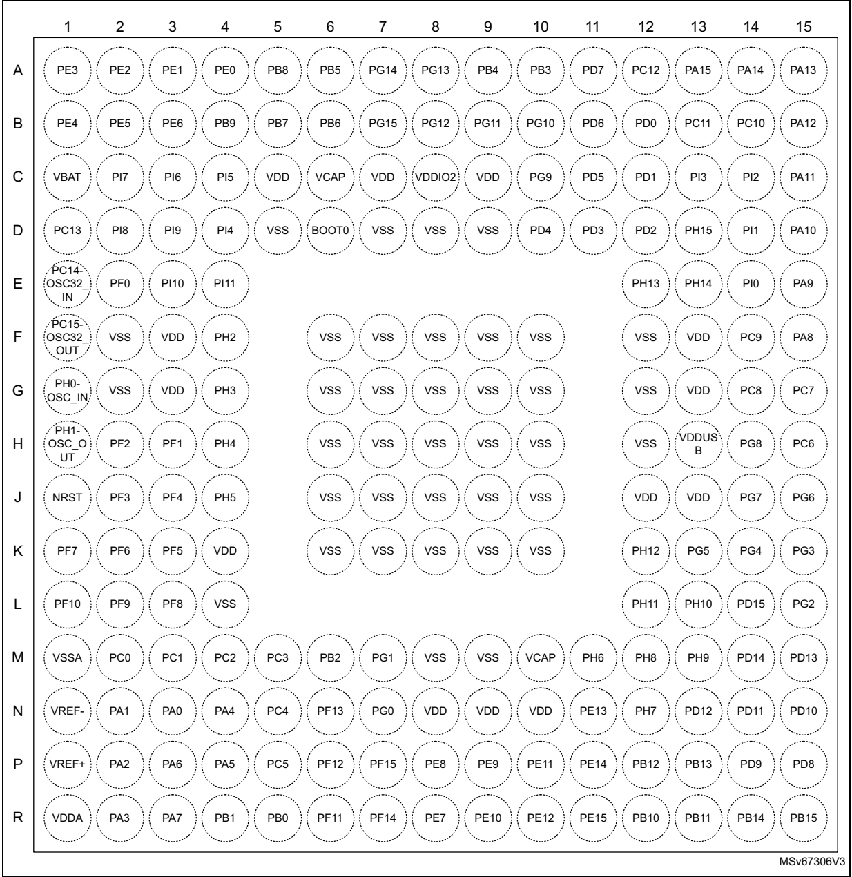
Figure 16. UFBGA176+25 ballout
