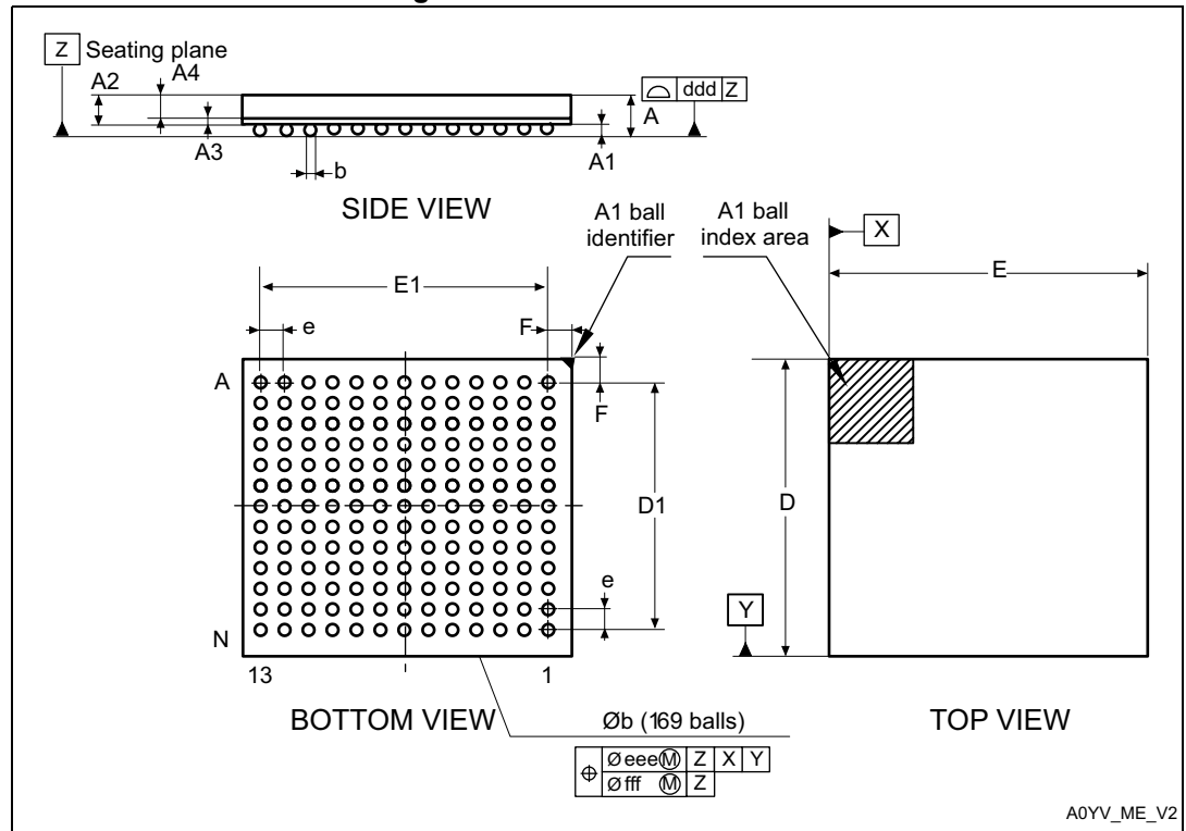
Figure 90. UFBGA169 - Outline
