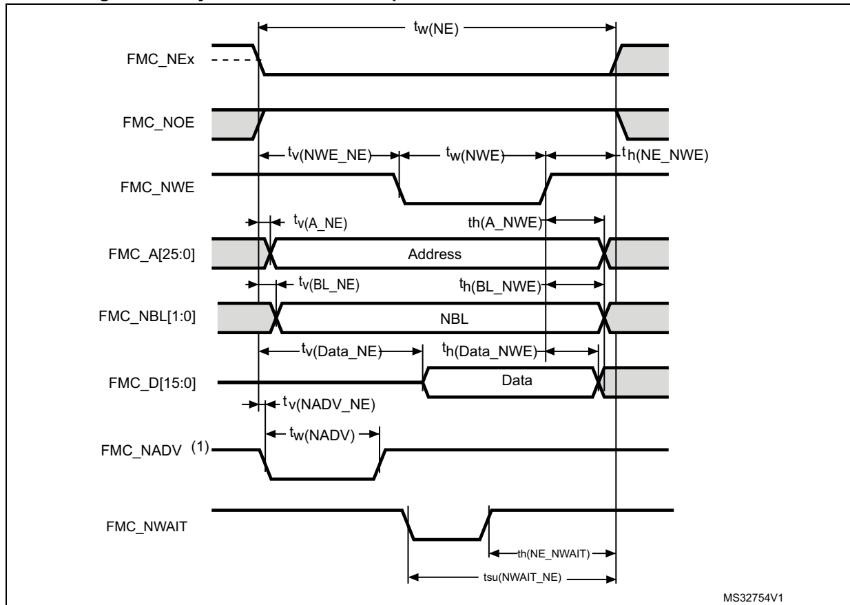
Figure 52. Asynchronous non-multiplexed SRAM/PSRAM/NOR write waveforms
