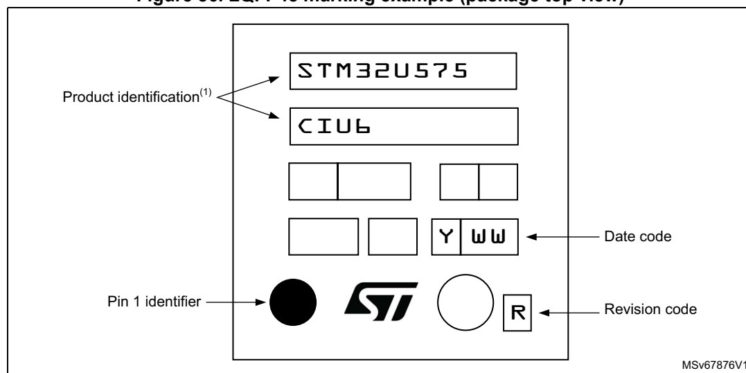
Figure 86. LQFP48 marking example (package top view)
