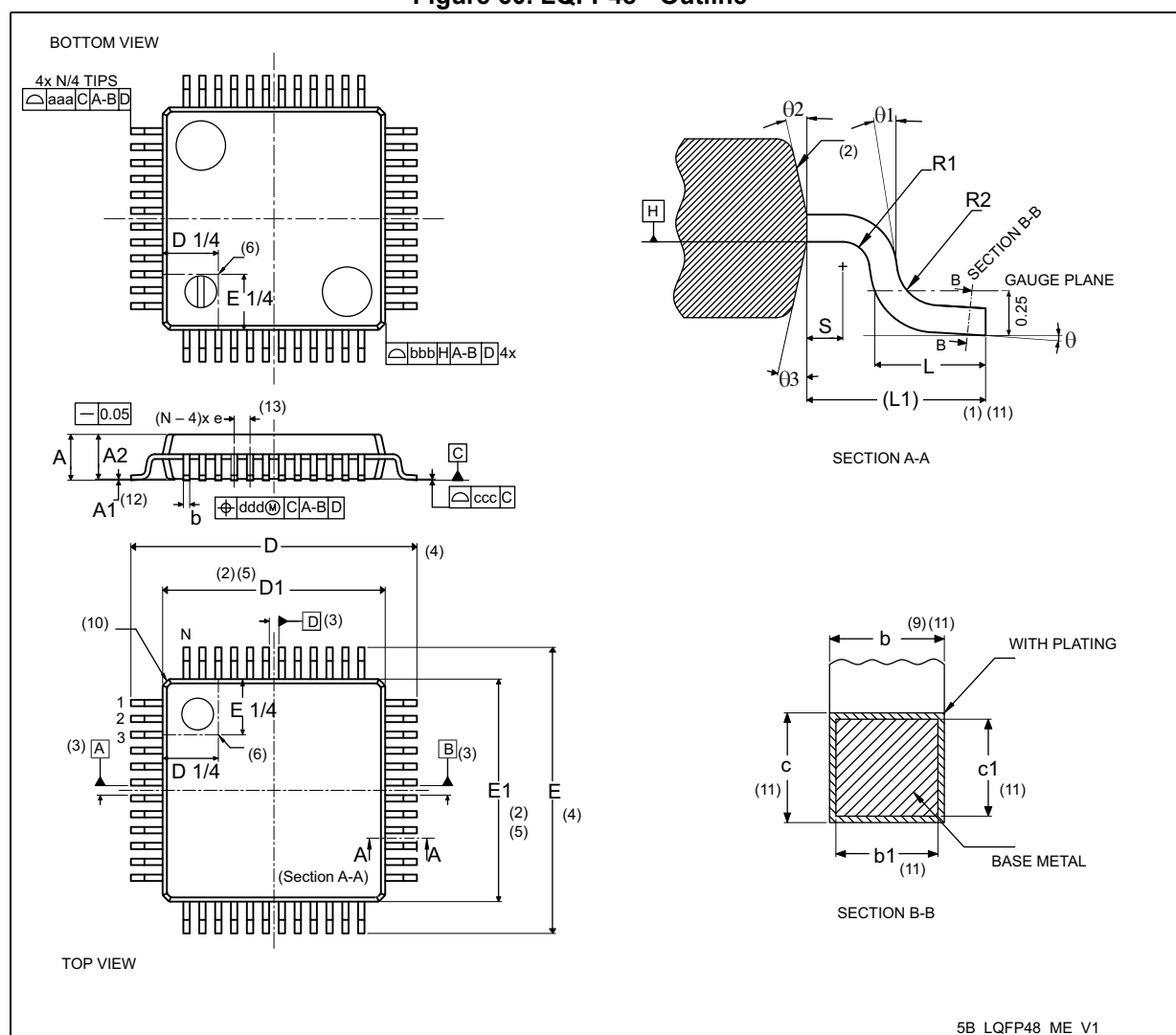
Figure 60. LQFP48 - Outline (15)
