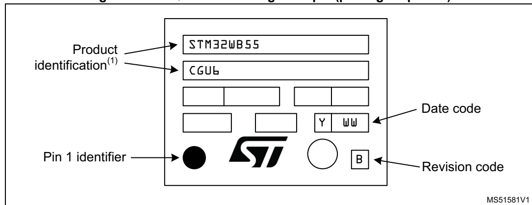
Figure 40. UFQFPN48 marking example (package top view)
