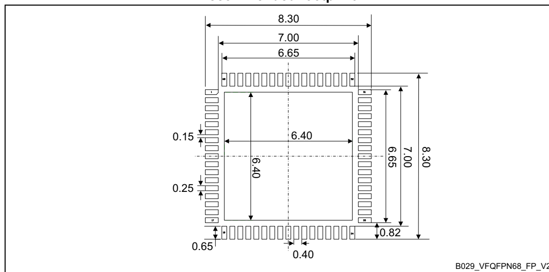
Figure 37. VFQFPN68, 8 x 8 mm, 0.4 mm pitch, very thin fine pitch quad flat recommended footprint
