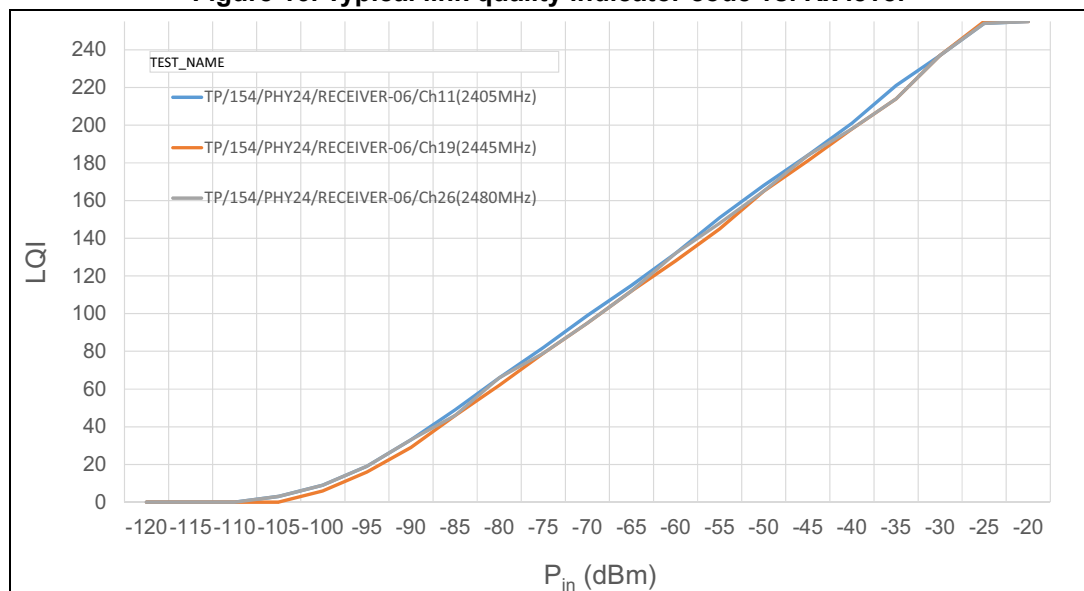
Figure 16. Typical link quality indicator code vs. Rx level
