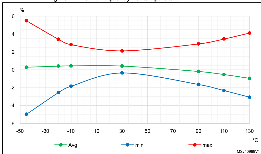
Figure 22. HSI48 frequency vs. temperature
