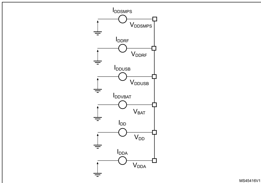
Figure 15. Current consumption measurement scheme
