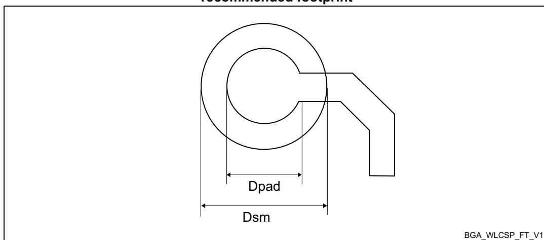
Figure 35. UFBGA - 129 balls, 7 x 7 mm, 0.5 mm fine pitch, square ball grid array recommended footprint
