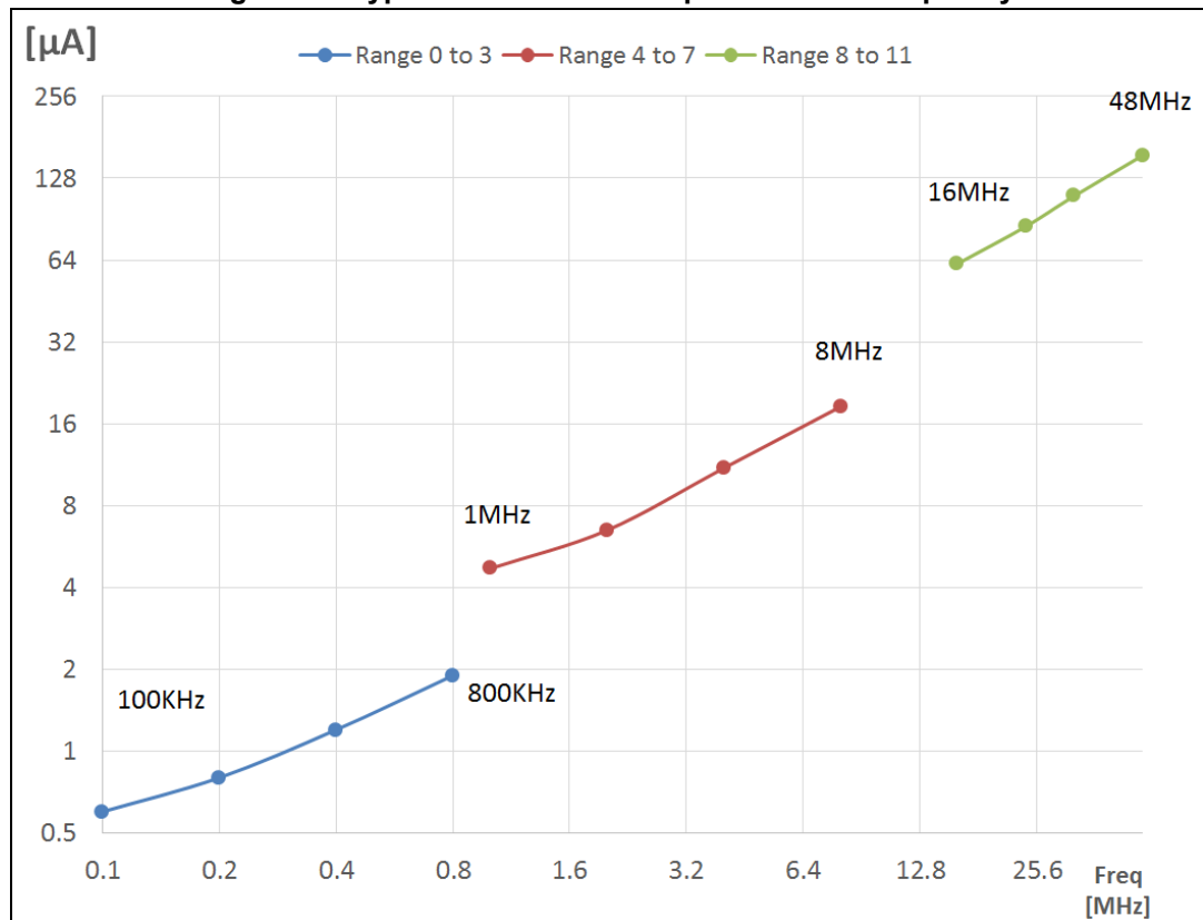
Figure 21. Typical current consumption vs. MSI frequency
