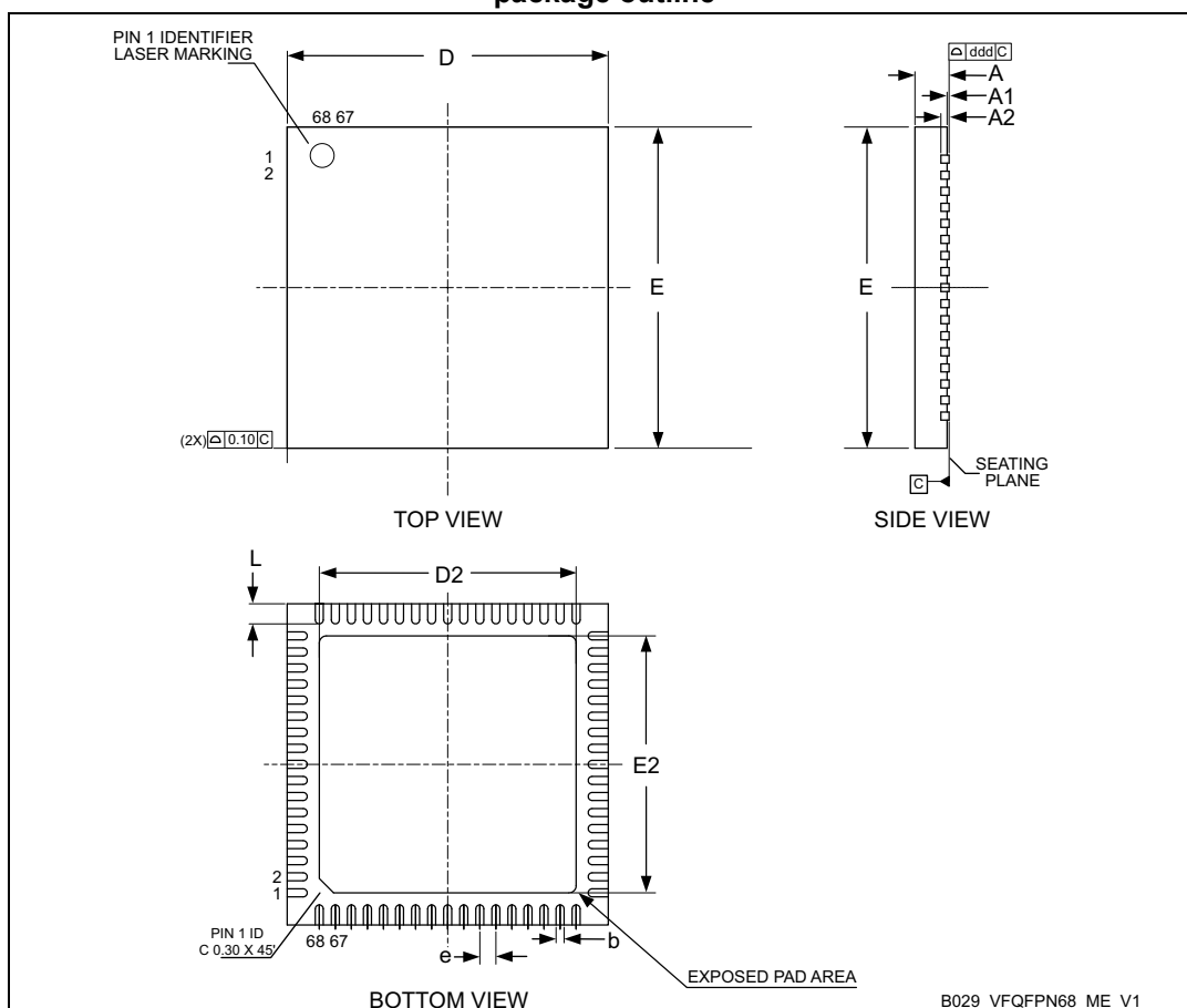
Figure 36. VFQFPN68, 8 x 8 mm, 0.4 mm pitch, very thin fine pitch quad flat package outline
