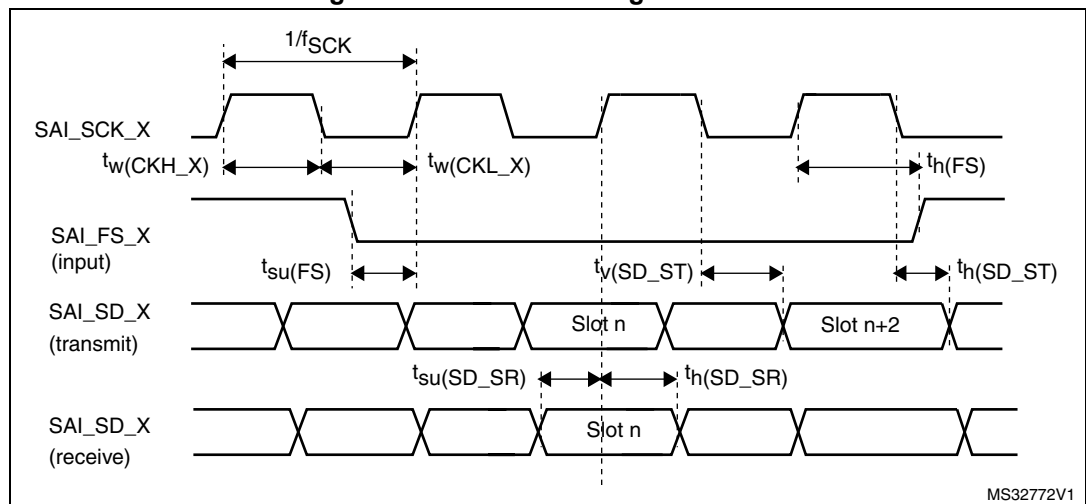
Figure 33. SAI slave timing waveforms
