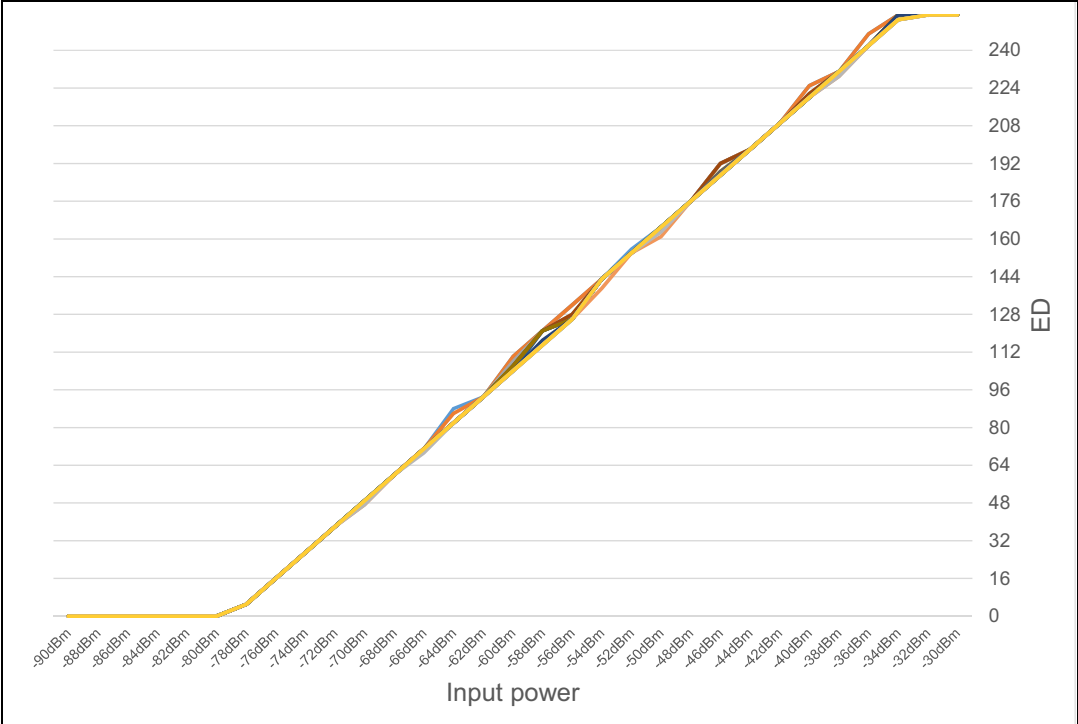
Figure 17. Typical energy detection (T = 27°C, V DD = 3.3 V)
