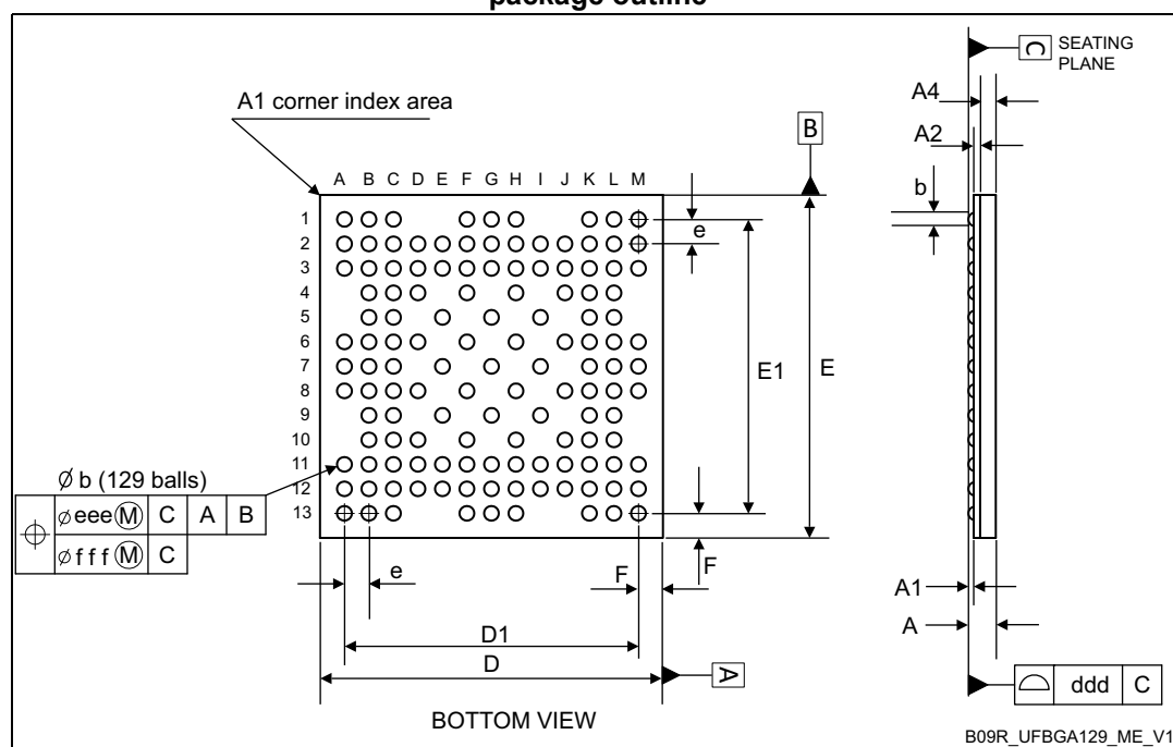
Figure 34. UFBGA - 129 balls, 7 x 7 mm, 0.5 mm fine pitch, square ball grid array package outline
