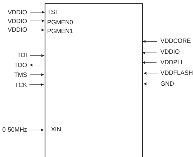
Figure 20-4. Serial Programming
