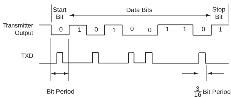
Figure 33-24. IrDA Modulation
