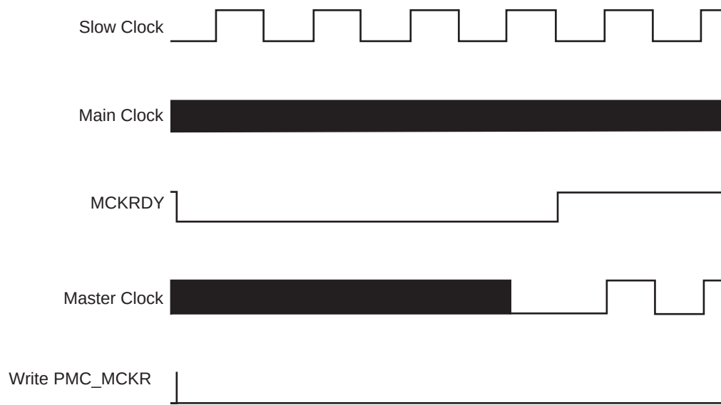
Figure 29-4. Switch Master Clock from Main Clock to Slow Clock
