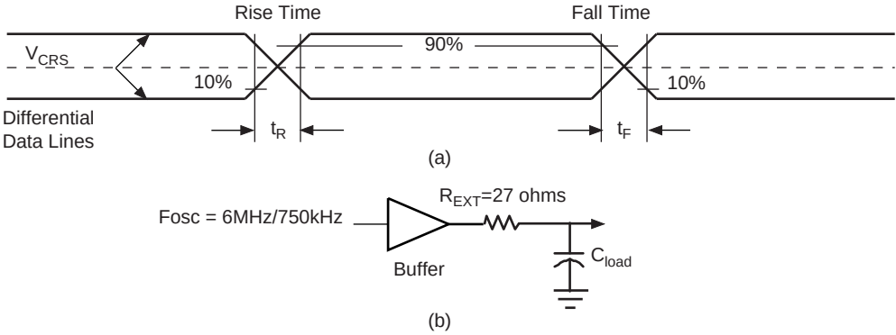
Figure 37-3. USB Data Signal Rise and Fall Times
