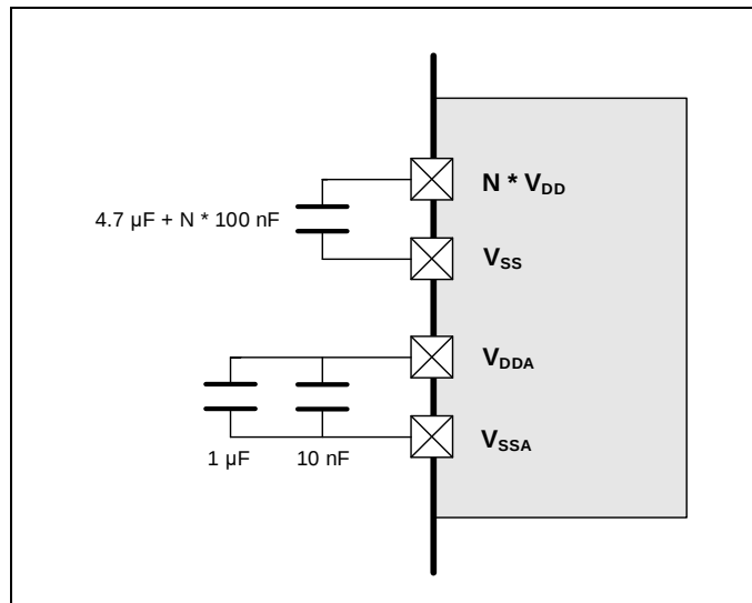
Figure 4-1. Recommended power supply decoupling capacitors (1)
