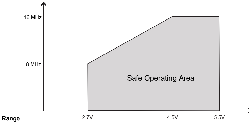
Figure 33-2. Maximum Frequency vs. V_{DD} for [-40, 125]^{\circ}\text{C} , Extended Temperature
