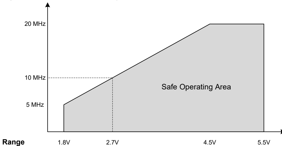
Figure 33-2. Maximum Frequency vs. V_{DD} for [-40, 125]^{\circ}\text{C} , Extended Temperature
