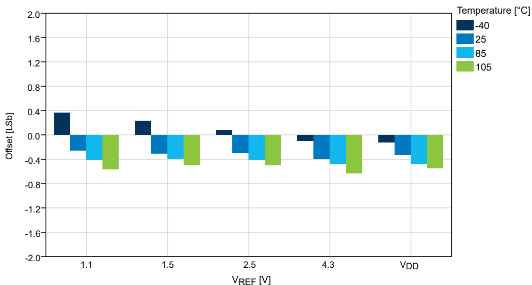
Figure 32-49. Offset Error vs. V_{REF} ( V_{DD} = 5.0V , f_{ADC} = 115 kps), REFSEL = Internal Reference
