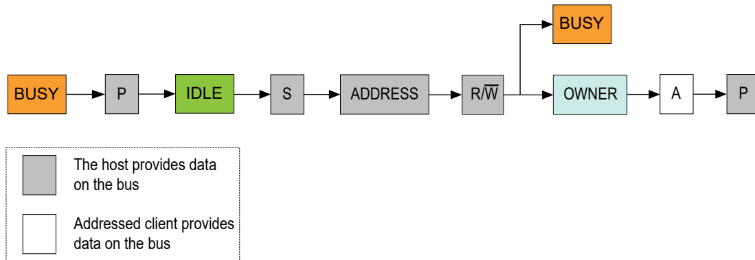
Figure 25-8. Quick Command Frame Format
