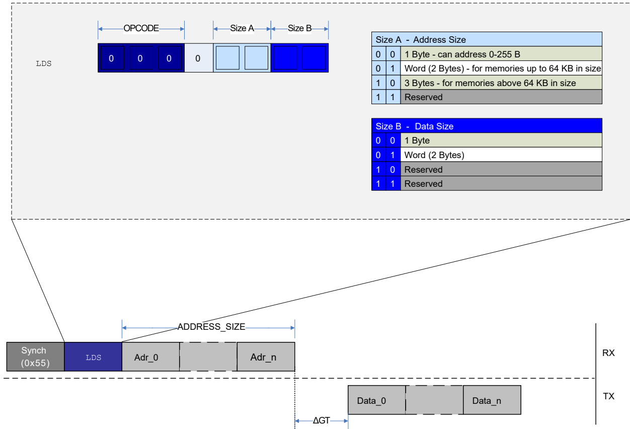
Figure 30-8. LDS Instruction Operation
