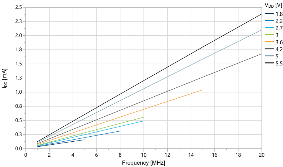
Figure 32-6. Idle Supply Current vs. Frequency (1-20 MHz) at T = 25^{\circ}C (EXTCLK)
