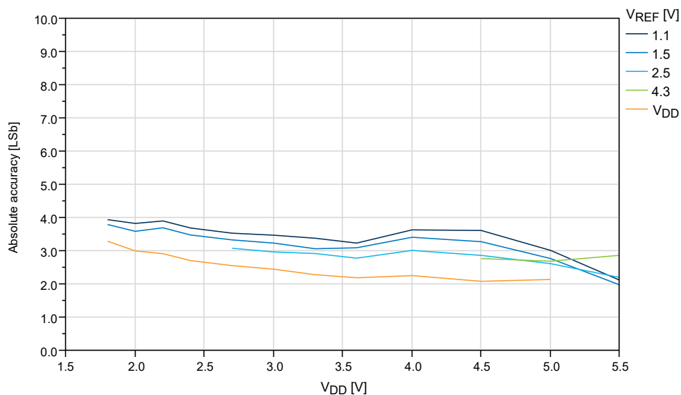
Figure 32-40. Absolute Accuracy vs. V_{DD} ( f_{ADC} = 115 kps) at T = 25^{\circ}\text{C} , REFSEL = Internal Reference
