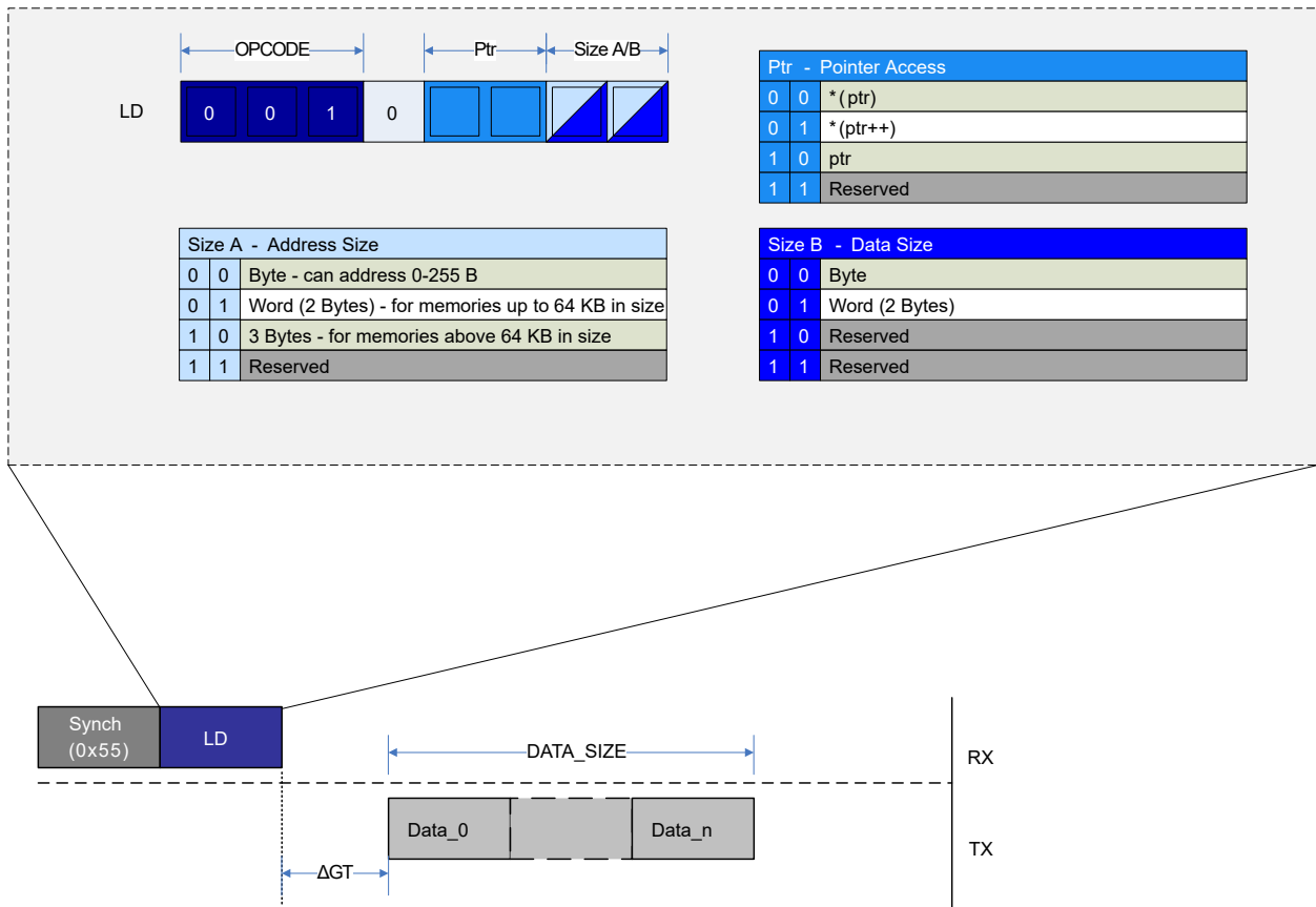
Figure 30-10. LD Instruction Operation
