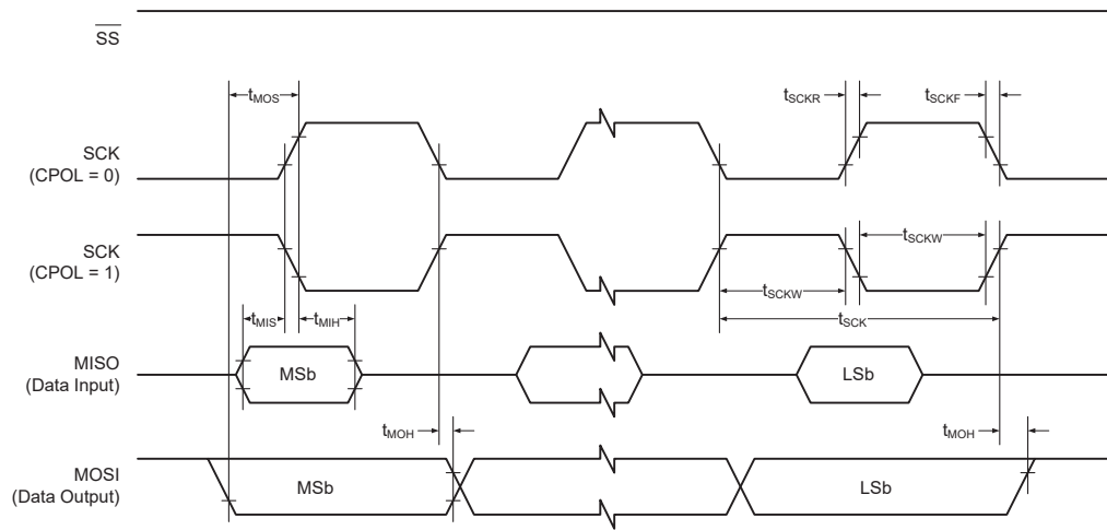
Figure 31-6. SPI - Timing Requirements in Client Mode
