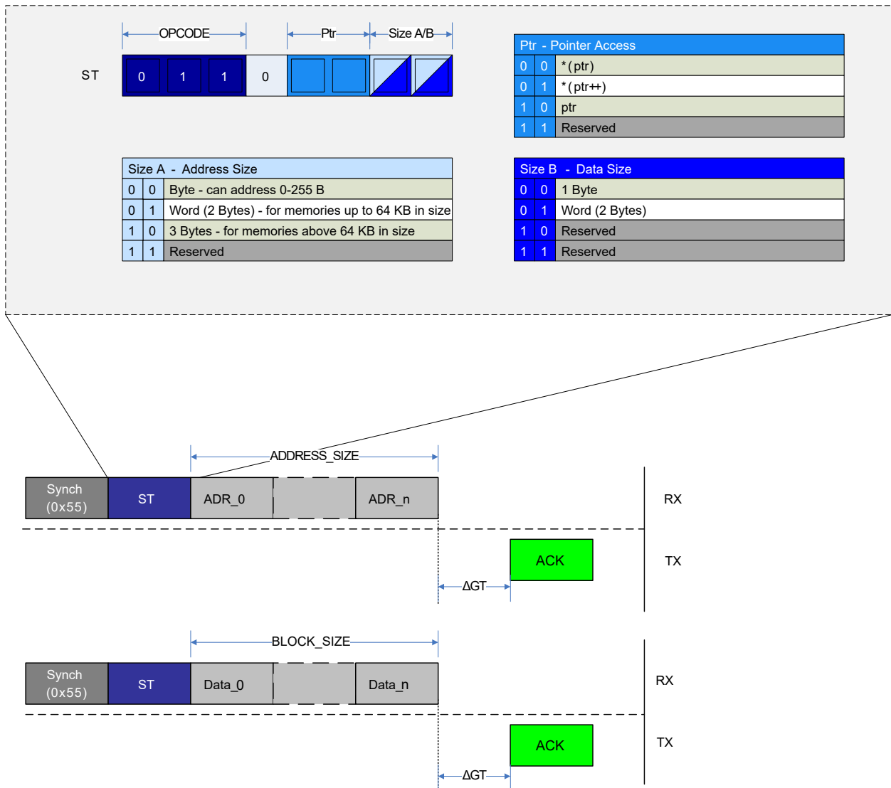
Figure 30-11. ST Instruction Operation
