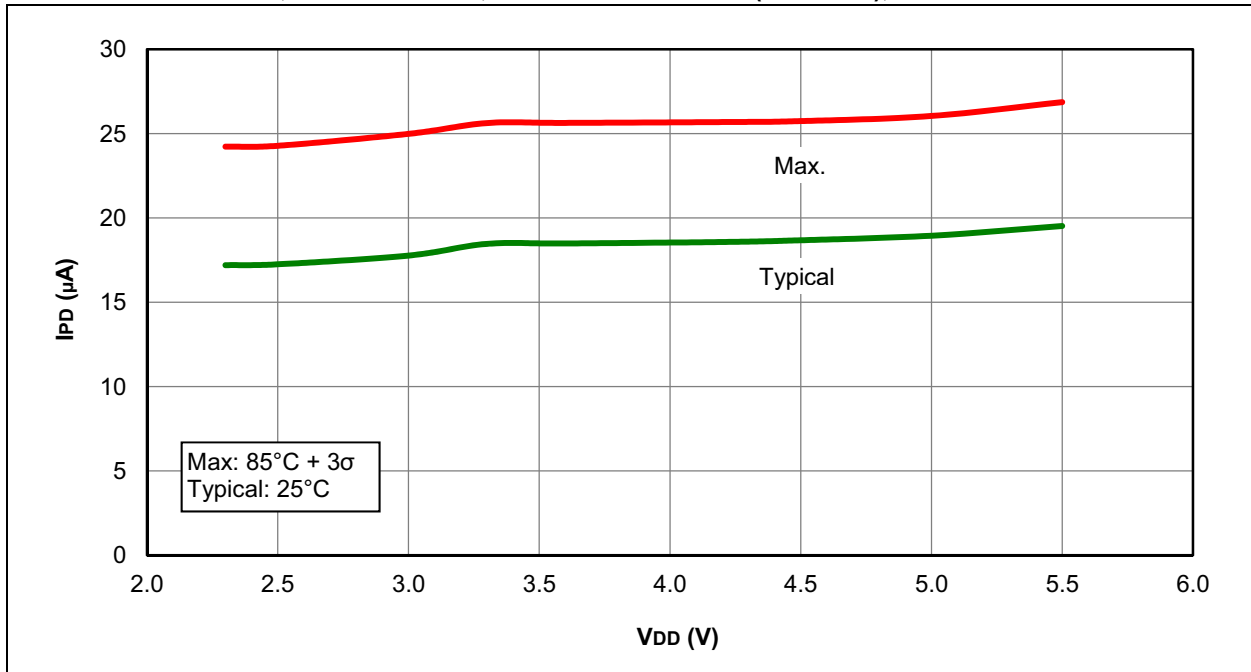
FIGURE 29-32: I_{PD} , COMPARATOR, LOW-POWER MODE ( C_{xSP} = 0 ), PIC16F1503 ONLY
