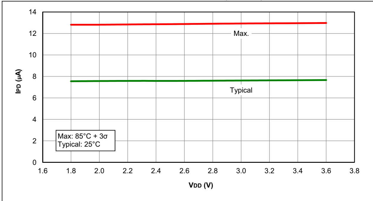
FIGURE 29-31: I_{PD} , COMPARATOR, LOW-POWER MODE ( C_{xSP} = 0 ), PIC16LF1503 ONLY
