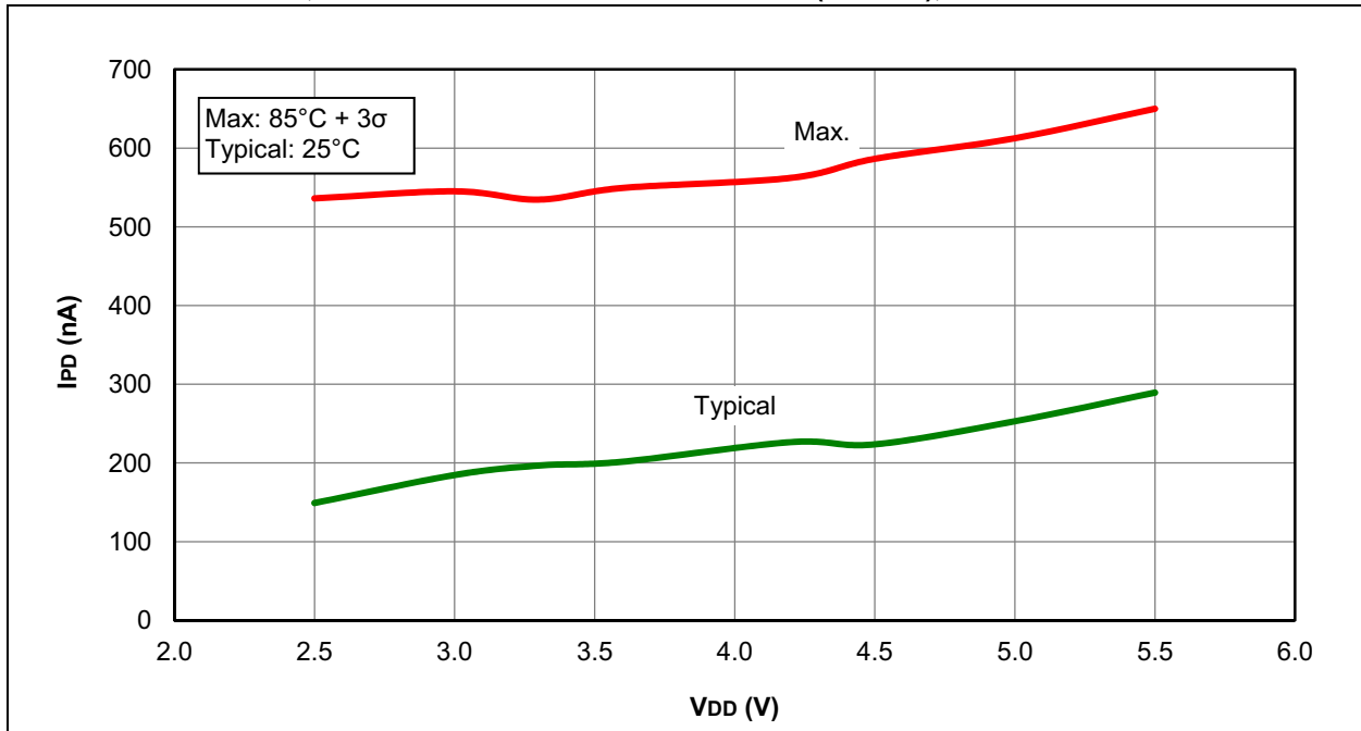
FIGURE 31-8: I_{PD} , LOW-POWER BROWN-OUT RESET (LPBOR), PIC16F1782/3 ONLY
