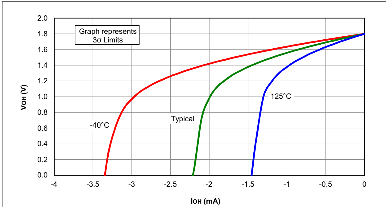
FIGURE 31-15: I_{PD} , V_{OL} vs. I_{OH} OVER TEMPERATURE, V_{DD} = 1.8V , PIC16LF1782/3 ONLY
