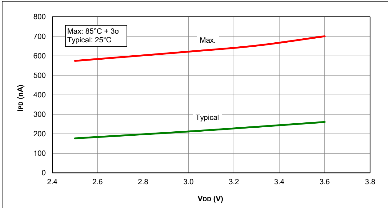
FIGURE 31-7: I_{PD} , LOW-POWER BROWN-OUT RESET (LPBOR), PIC16LF1782/3 ONLY
