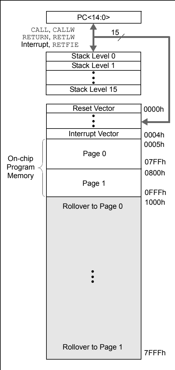
FIGURE 3-2: PROGRAM MEMORY MAP AND STACK FOR PIC16F1783
