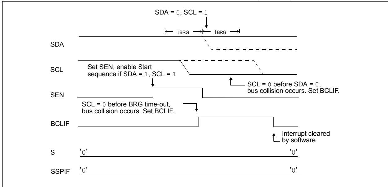
FIGURE 27-35: BRG RESET DUE TO SDA ARBITRATION DURING START CONDITION
