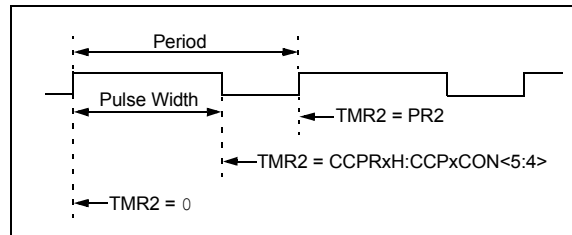
FIGURE 26-3: CCP PWM OUTPUT SIGNAL
