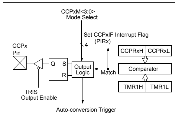
FIGURE 26-2: COMPARE MODE OPERATION BLOCK DIAGRAM
