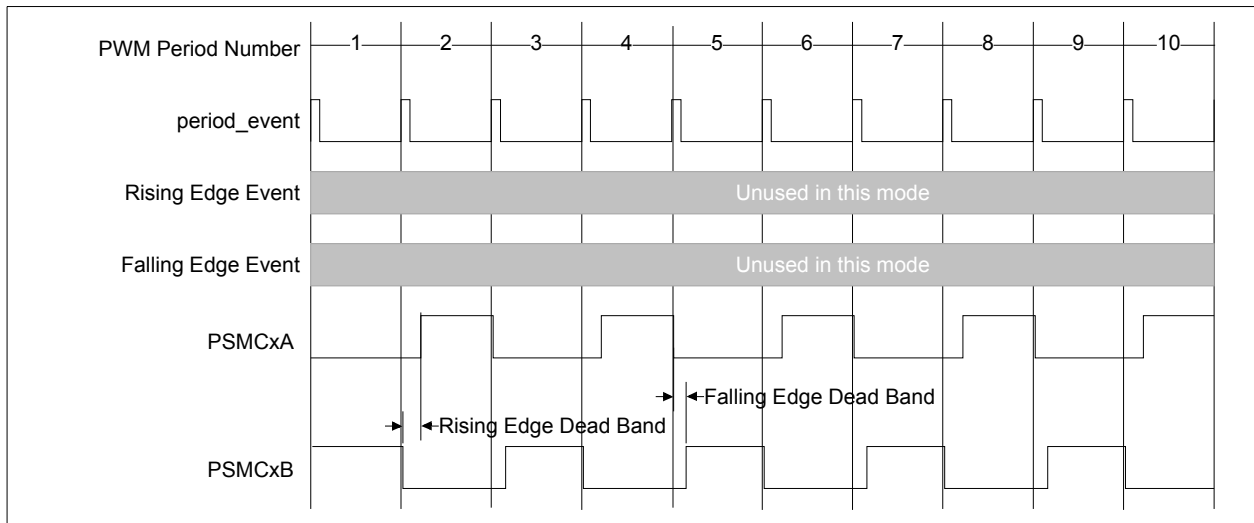
FIGURE 25-14: VARIABLE FREQUENCY – FIXED DUTY CYCLE PWM WITH COMPLEMENTARY OUTPUTS WAVEFORM
