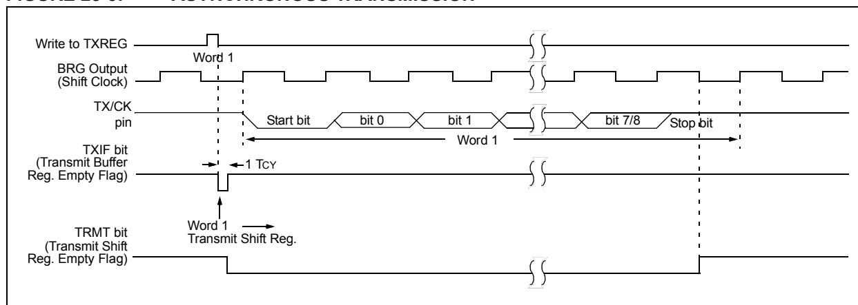
FIGURE 28-3: ASYNCHRONOUS TRANSMISSION
