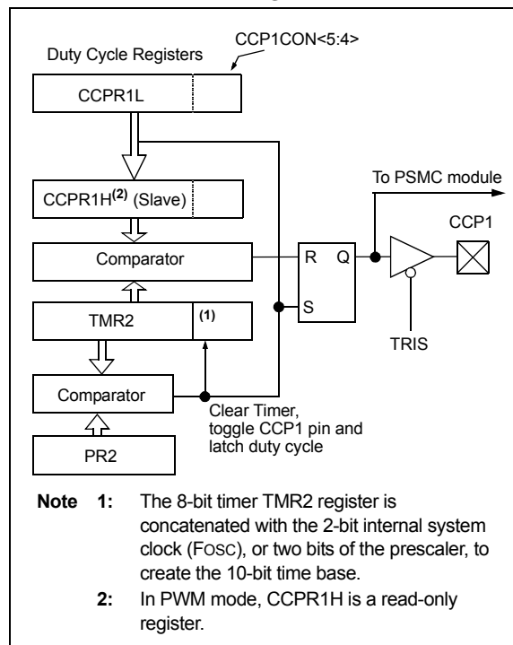
FIGURE 26-4: SIMPLIFIED PWM BLOCK DIAGRAM
