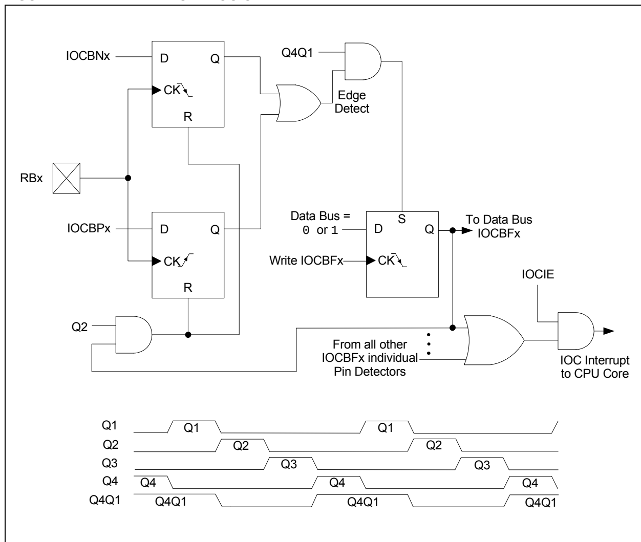
FIGURE 7-1: INTERRUPT LOGIC
