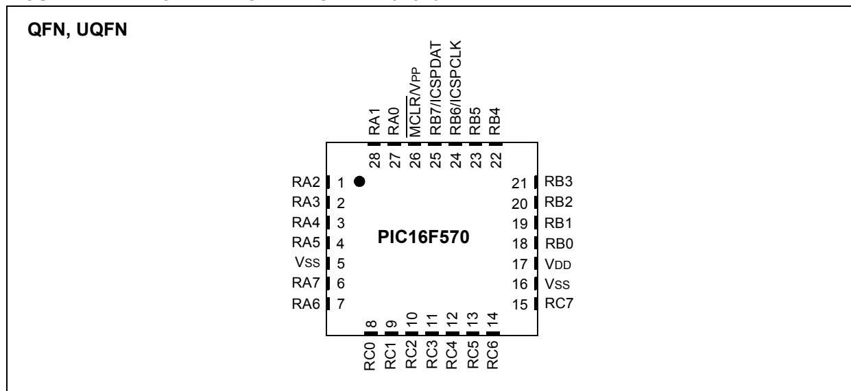
FIGURE 2: 28-PIN DIAGRAM FOR PIC16F570
