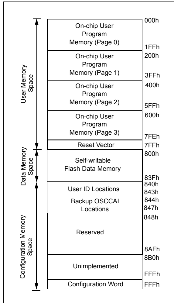
FIGURE 4-1: MEMORY MAP
