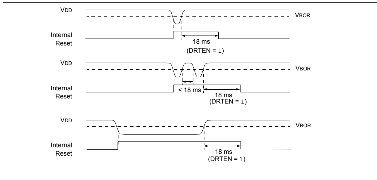
FIGURE 8-13: BROWN-OUT SITUATIONS
