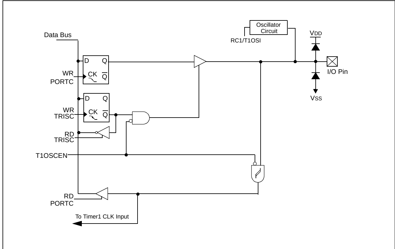
FIGURE 6-13: BLOCK DIAGRAM OF RC0
