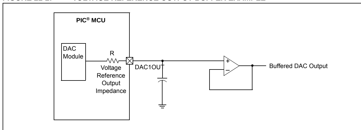
FIGURE 21-2: VOLTAGE REFERENCE OUTPUT BUFFER EXAMPLE
