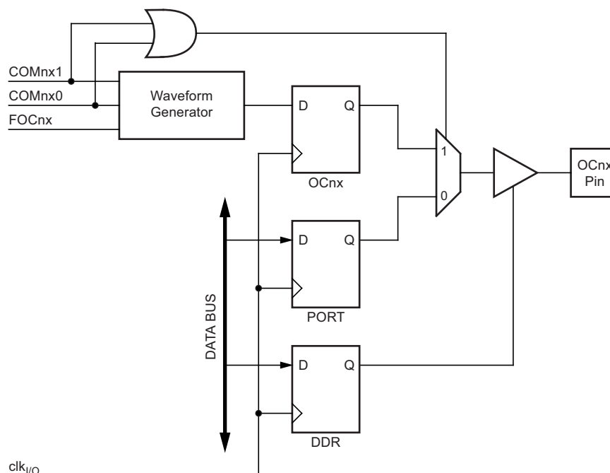
Figure 14-4. Compare Match Output Unit, Schematic
