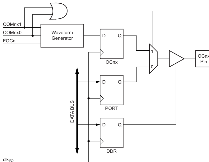
Figure 15-5. Compare Match Output Unit, Schematic
