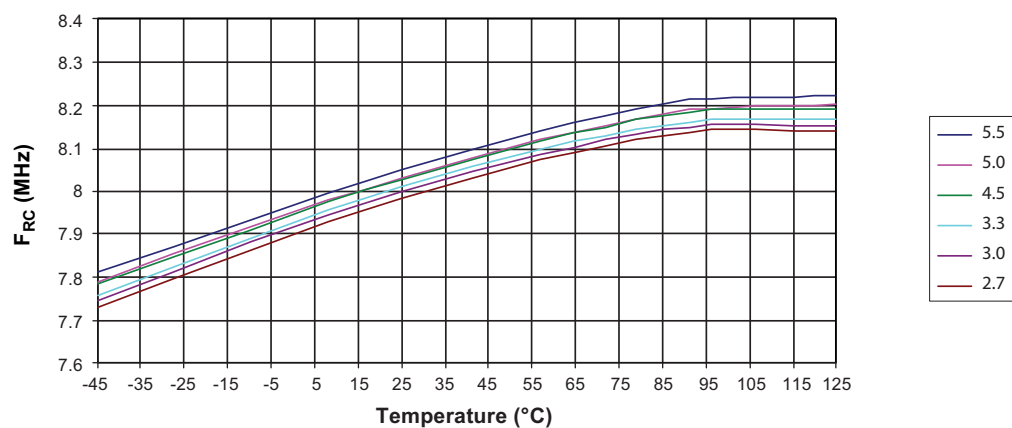
Figure 29-18. Calibrated 8MHz RC Oscillator Frequency versus Temperature
