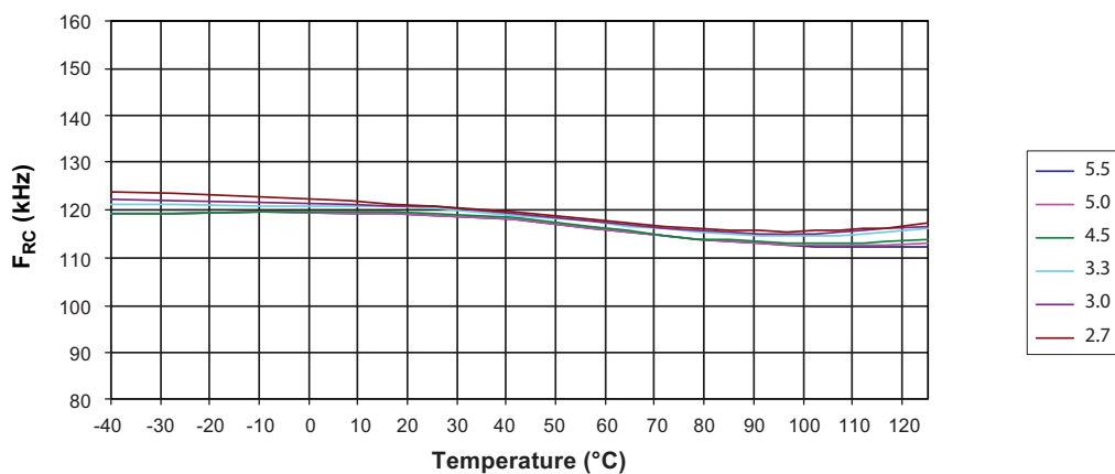
Figure 29-17. Watchdog Oscillator Frequency versus Temperature
