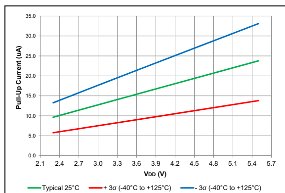
FIGURE 38-89: Weak Pull-up Current, PIC16F18856/76 Only.
