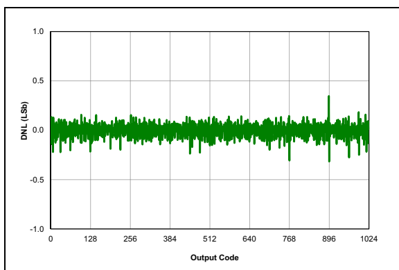
FIGURE 38-33: ADC, DNL, V_{DD} = 3.0V , T_{AD} = 1\text{ }\mu S , 25^\circ C .
