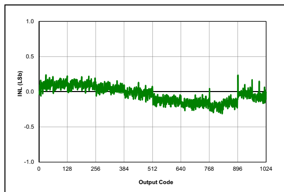
FIGURE 38-35: ADC, INL, V_{DD} = 3.0V , T_{AD} = 1\text{ }\mu S , 25^\circ C .
