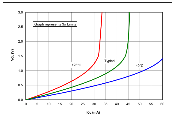
FIGURE 38-4: V_{OL} vs. I_{OL} Over Temperature, V_{DD} = 3.0V .
