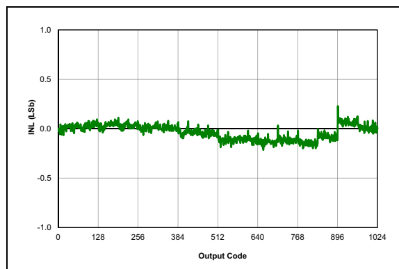
FIGURE 38-36: ADC, INL, V_{DD} = 3.0V , T_{AD} = 4\text{ }\mu S , 25^\circ C .
