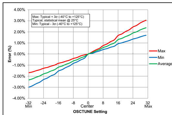
FIGURE 38-88: OSCTUNE Center Frequency, PIC16LF18856/76 Only.
