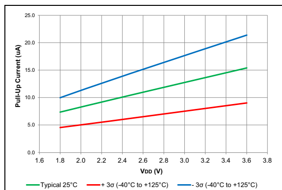
FIGURE 38-90: Weak Pull-up Current, PIC16LF18856/76 Only.
