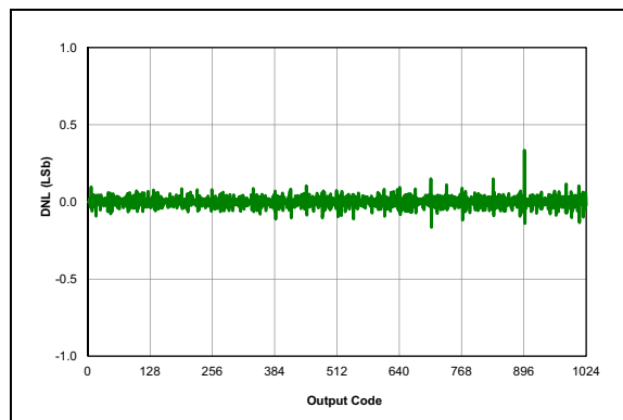
FIGURE 38-34: ADC, DNL, V_{DD} = 3.0V , T_{AD} = 4\text{ }\mu S , 25^\circ C .
