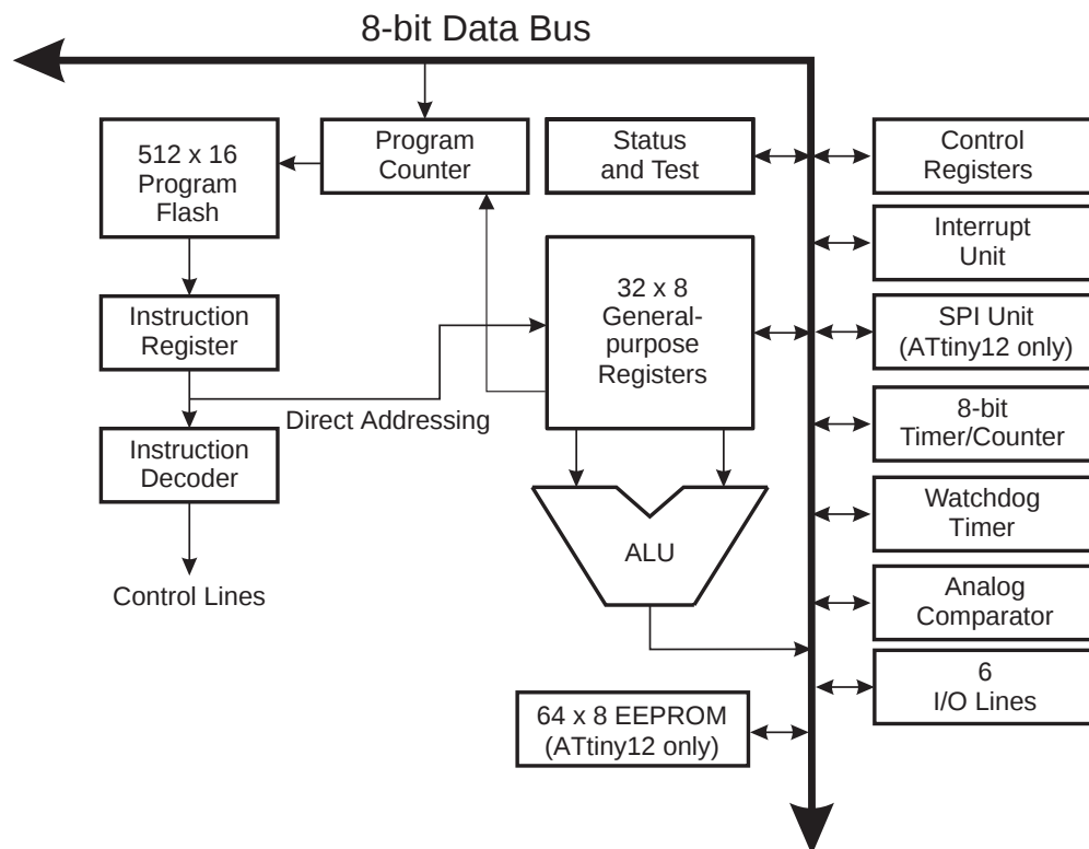
Figure 6. The ATtiny11/12 AVR RISC Architecture
