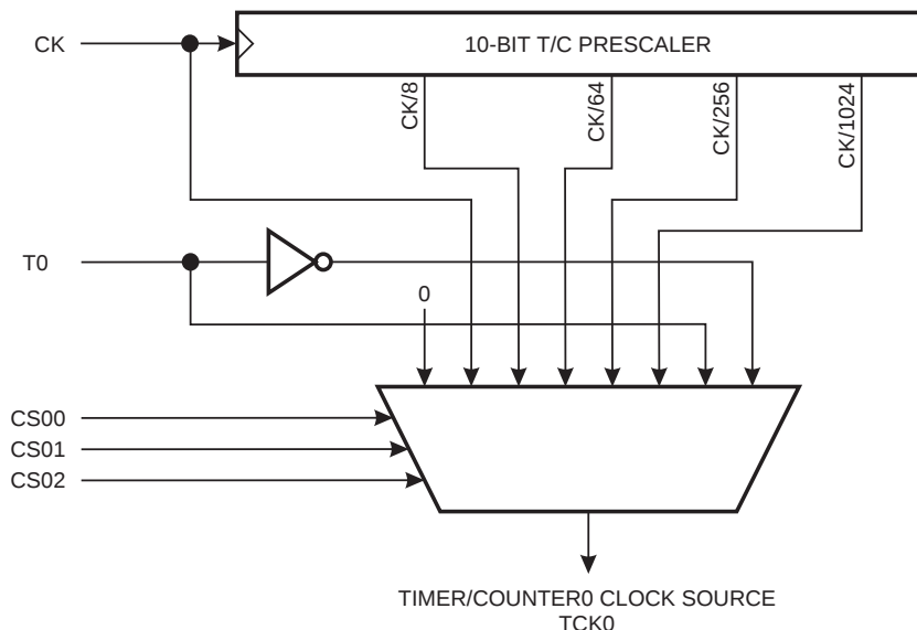
Figure 23. Timer/Counter0 Prescaler
