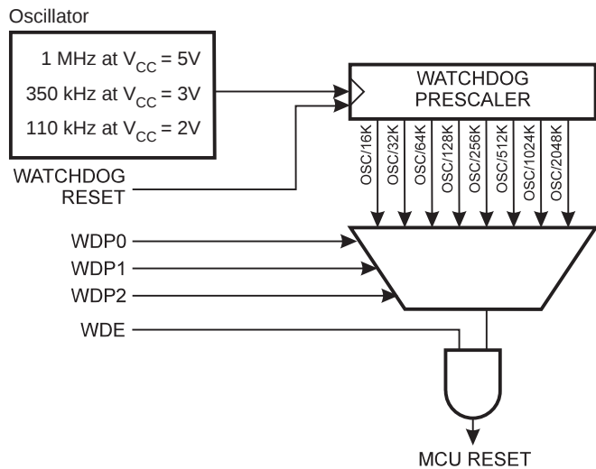
Figure 25. Watchdog Timer
