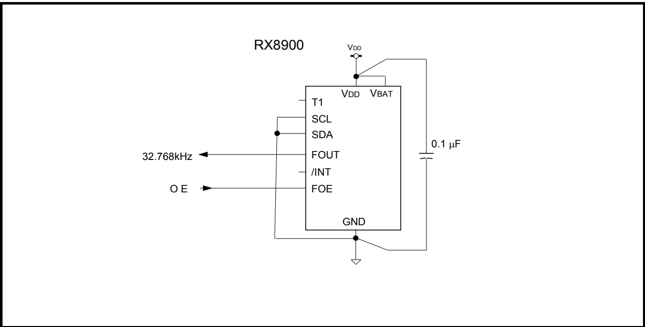
Figure 8-39. Connection RTC used as a clock source (32 kHz-TCXO)
