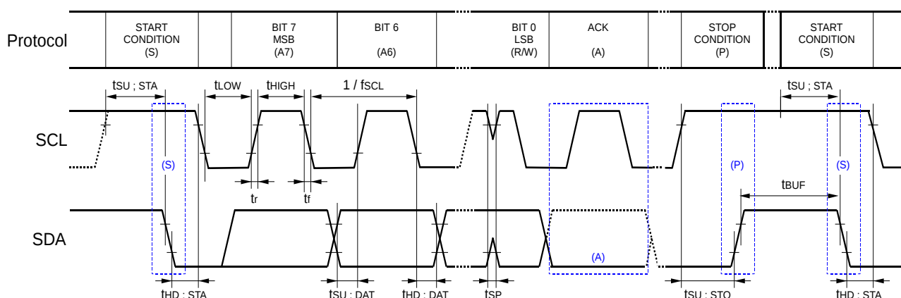
Timing chart
