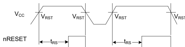
Figure 2. Power Fail nRESET Timing
