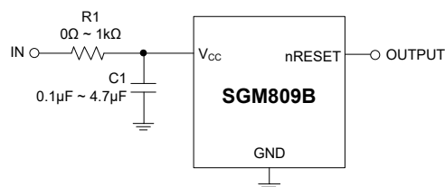
Figure 3. Preventing the High Voltage Spike
