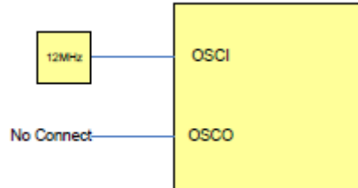
Figure 2.7 External Crystal Clock Source
