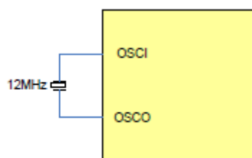
Figure 2.6 External Crystal
