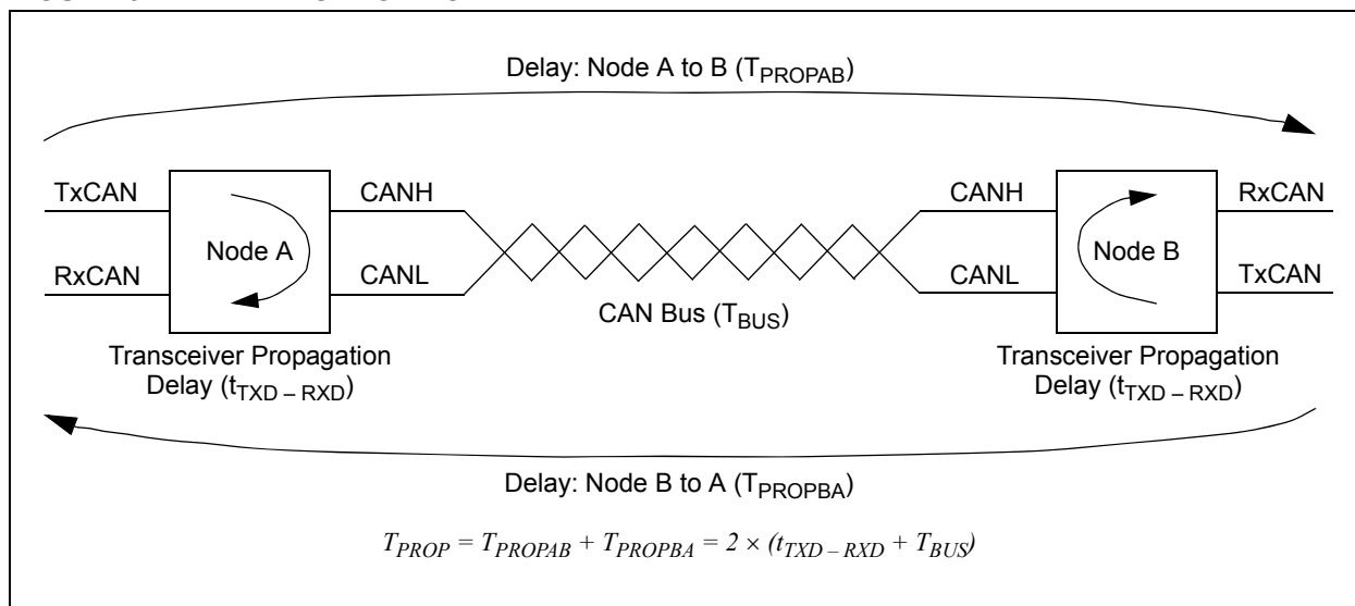
FIGURE 3-11: PROPAGATION DELAY
