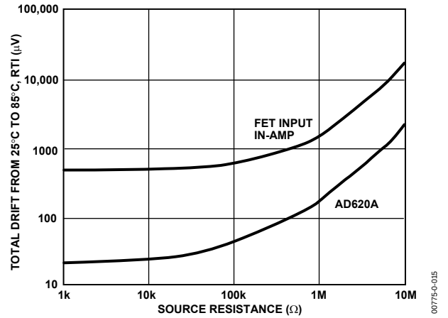
Figure 13. Total Drift vs. Source Resistance
