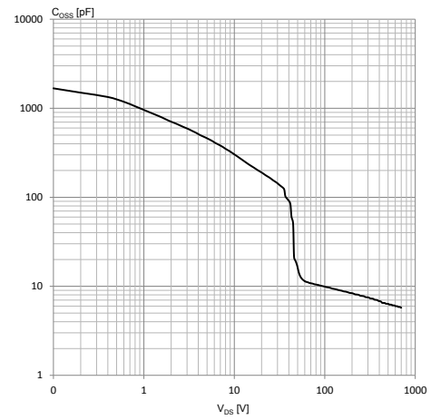
Figure 18. Power MOSFET C_{OSS} vs. V_{DS} @ V_{GS}=0 , f=1 MHz
