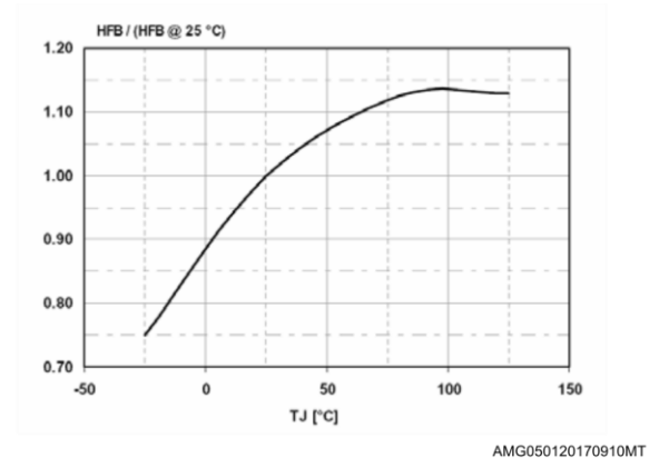
Figure 10: HFB vs T_J
