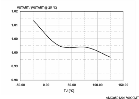
Figure 9: Drain start voltage vs T_J
